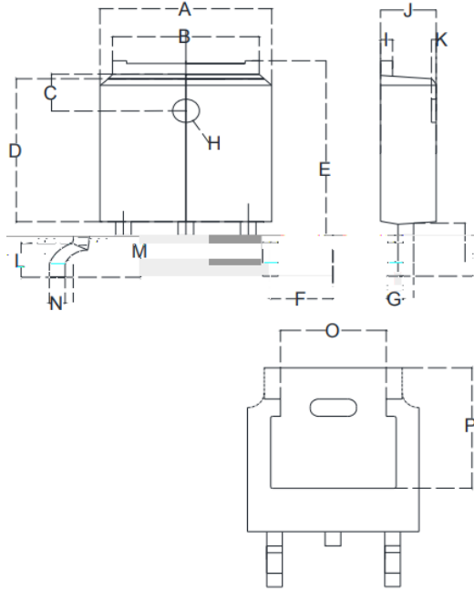
TO-252
